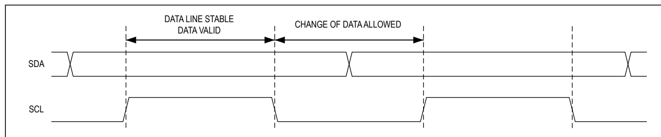
Figure 10. I 2 C Bit Transfer
